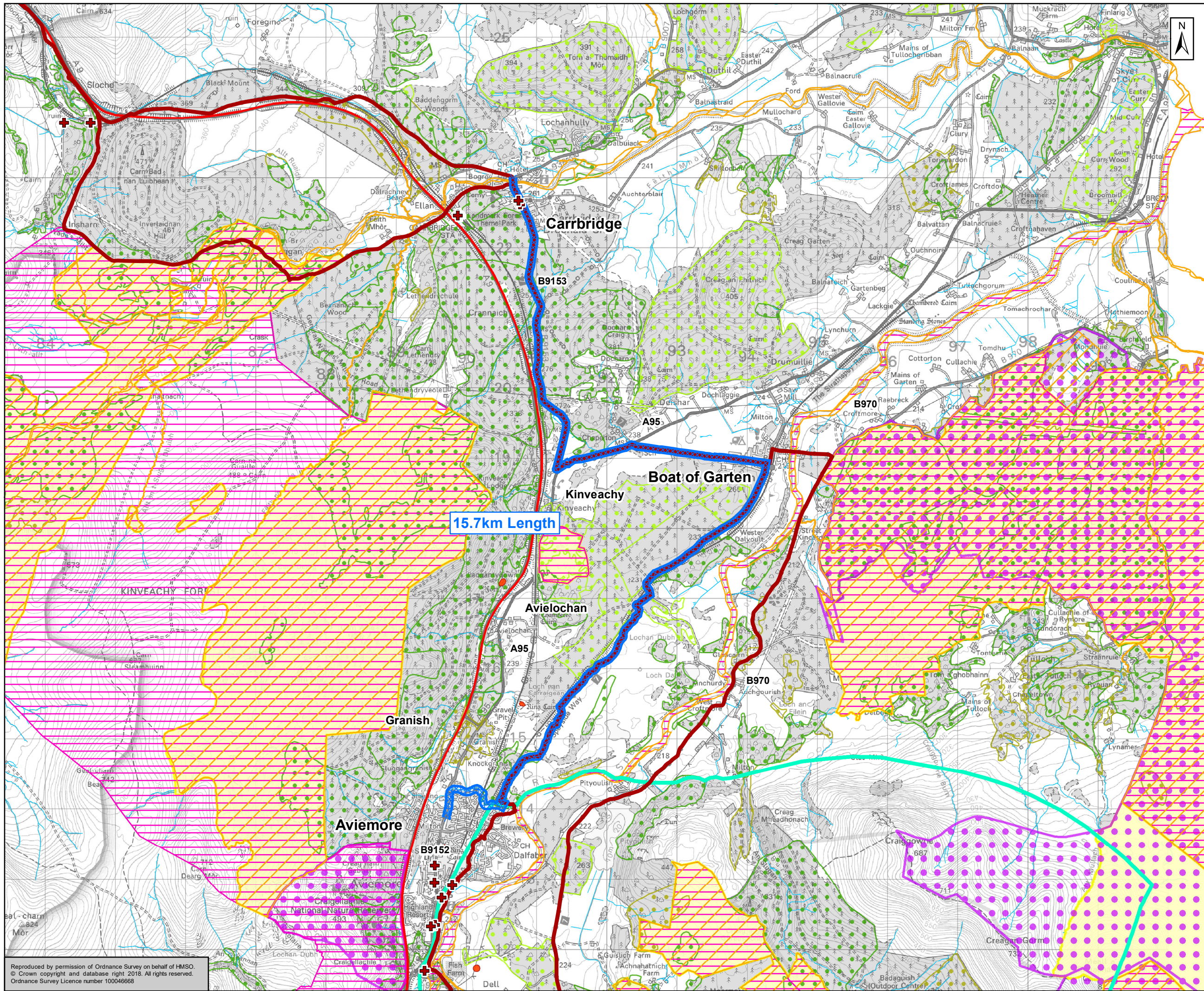
Figure 2.6 Identified Corridor Option 6 Segregated NMU Sheet 1 of 1
