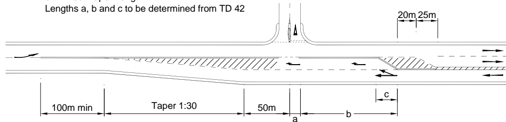
a) Right-turn at End of Single Lane Section
