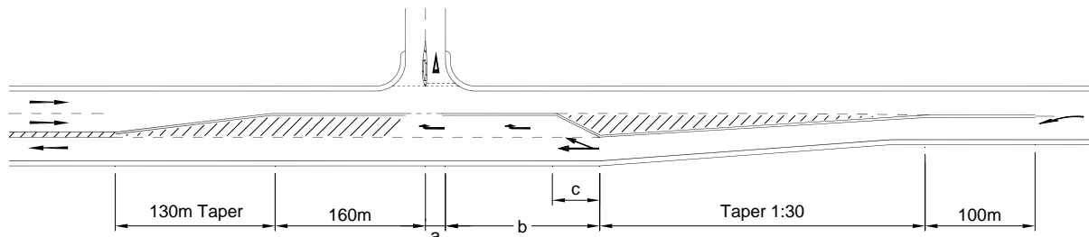
d) Right-turn at Start of Single Lane Section
