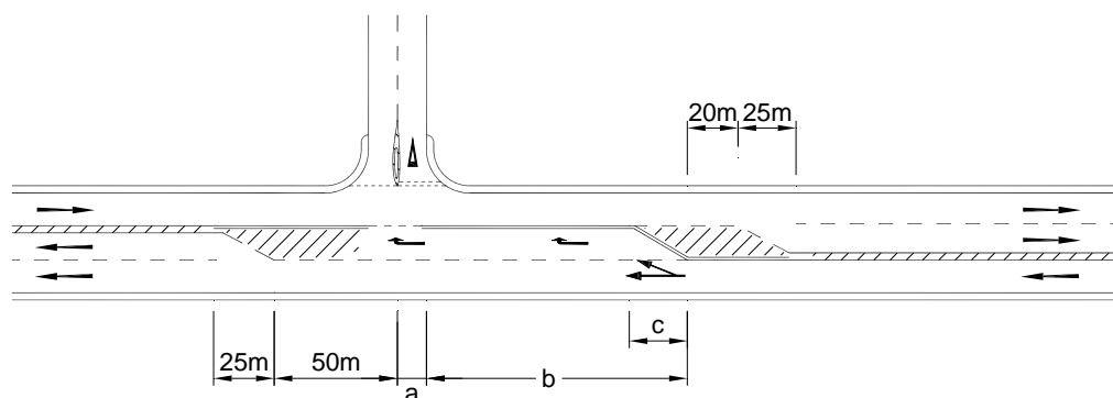
b) Non-conflicting Layout
