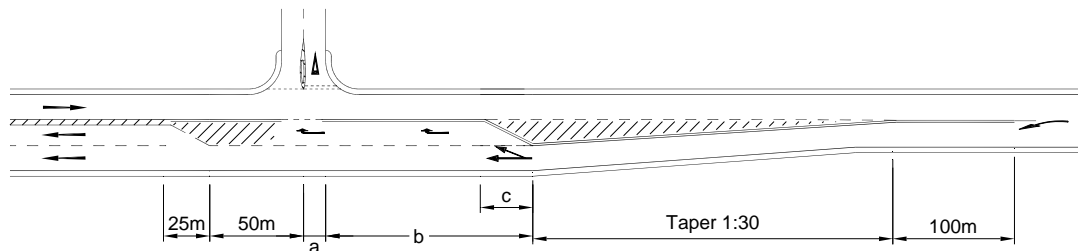
c) Right-turn at Start of Overtaking Lane Section
