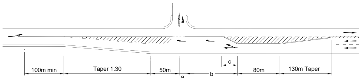
b) Right-turn at End of Overtaking Lane Section
