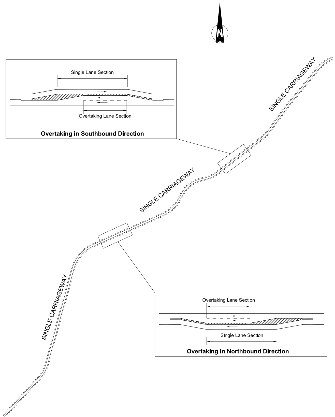
Figure 2/2: Individual Sections of WS2+1 Road Providing Overtaking Opportunities in One Direction
