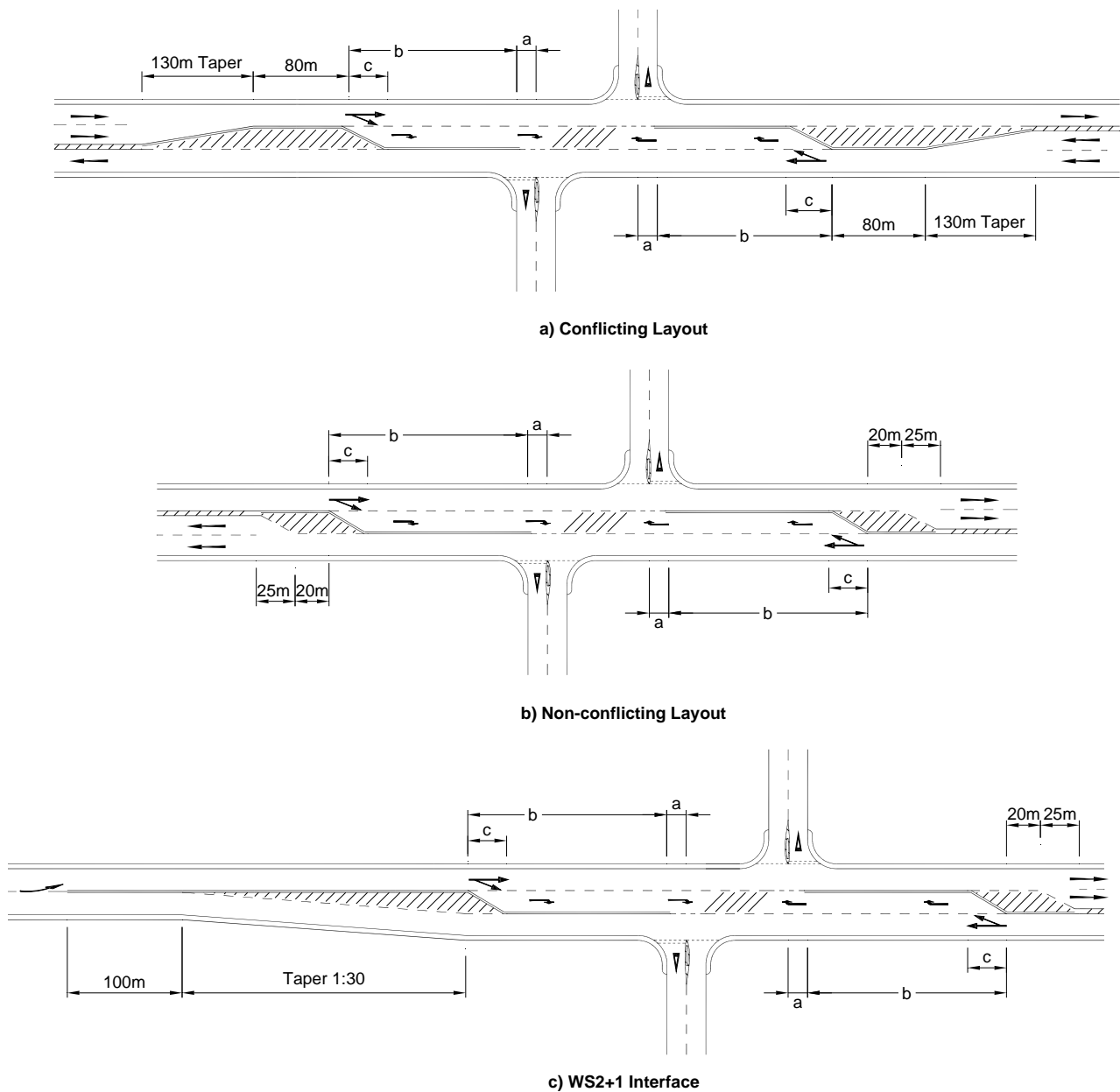
Figure 4/3: Staggered Junction Layouts at Changeovers & WS2+1 Interfaces
