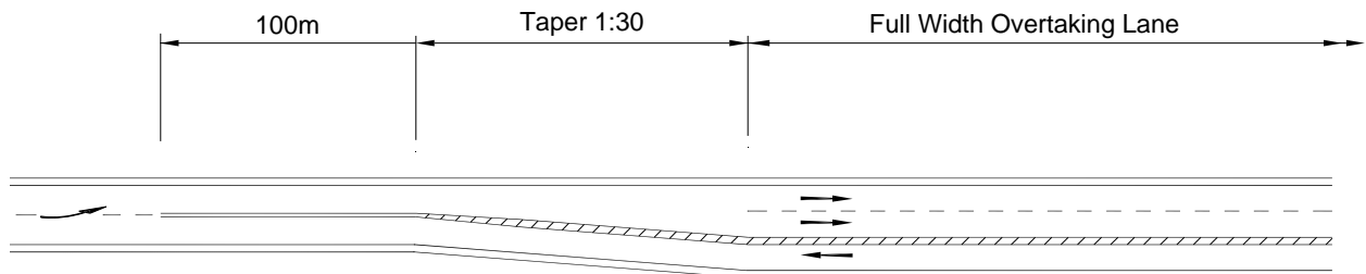
a) Start of Overtaking Lane Section with Widening on Right
