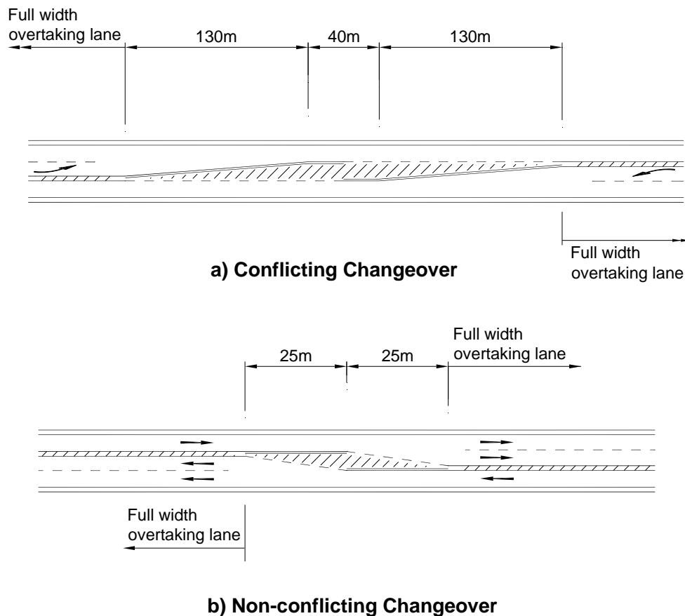
Figure 3/3: Dimensions of Changeovers
