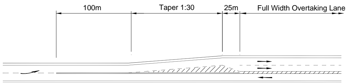
b) Start of Overtaking Lane Section with Widening on Left
