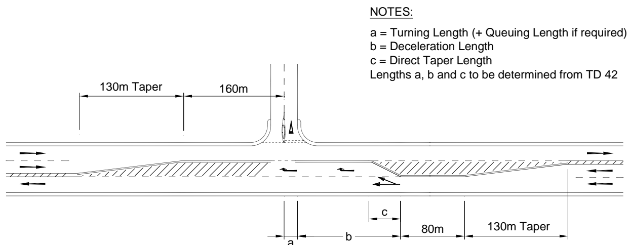
a) Conflicting Layout
