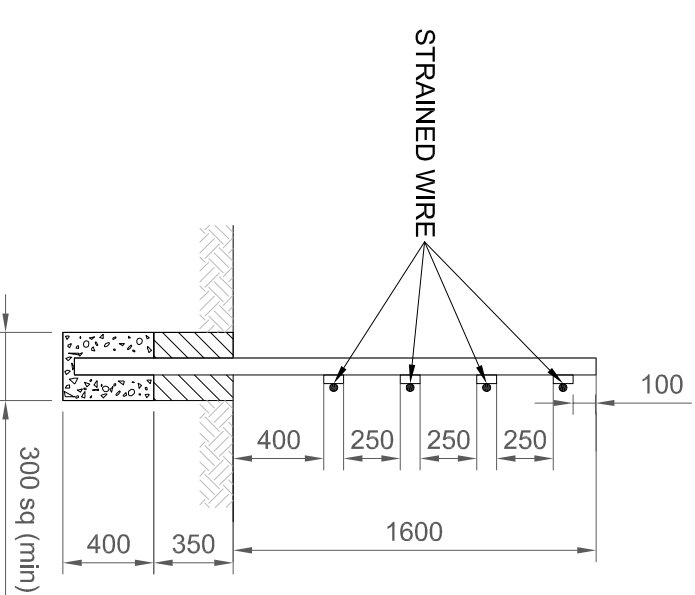
SECTION THROUGH CENTERLINE OF MAIN POSTS
