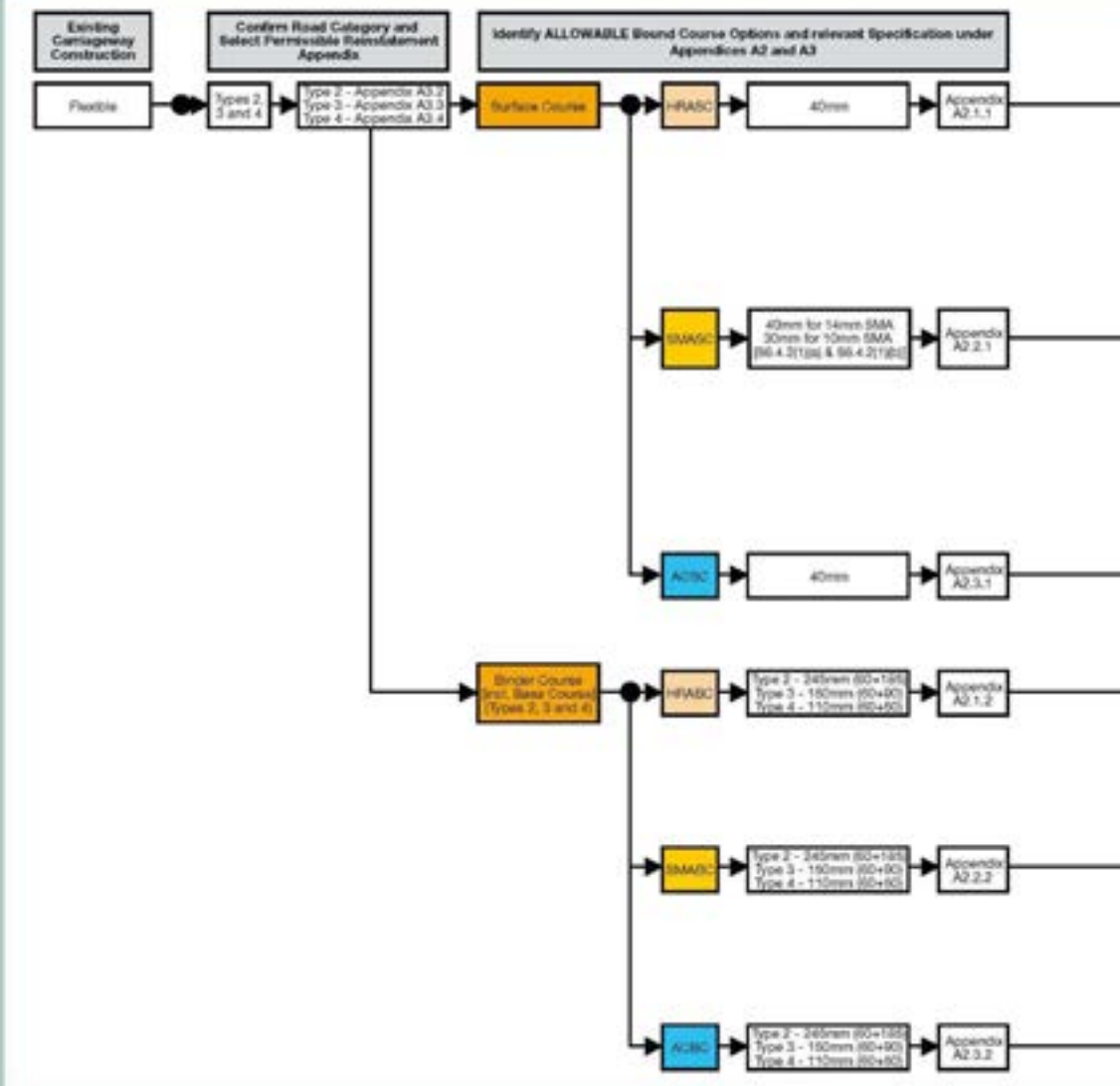
Figure A2.4 Permanent Reinstatement Options for Hot Lay Flexible Materials (Road Types 2, 3 and 4)
