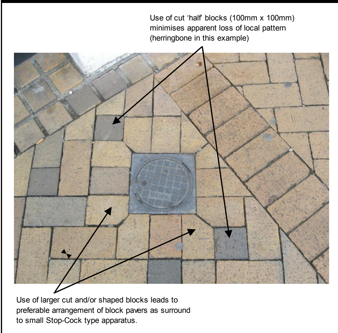
Figure NGA12.6 Acceptable Loss of Module Pattern - Modules up to 300mm [Picture 3]
