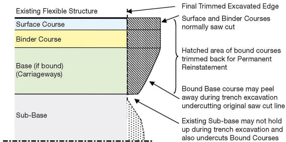
Figure S6.3 Example of Need for Trimback due to Undercutting
