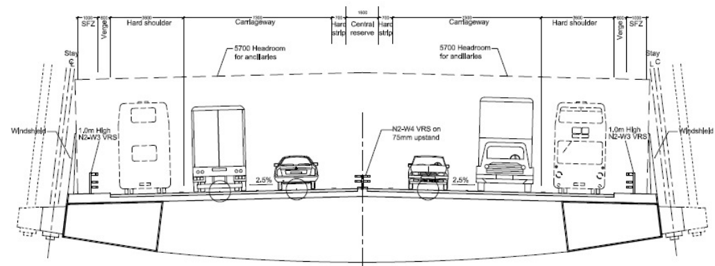
Cable Stay Deck at Main Span
