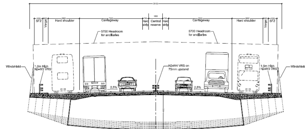
Approach Bridge Deck
