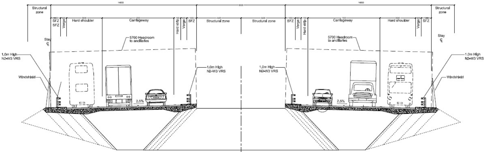
Approach Bridge Deck
