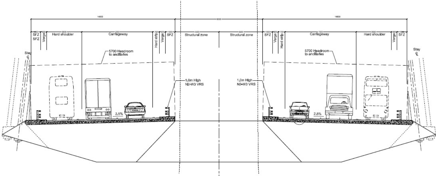
Cable Stay Deck at Main Span
