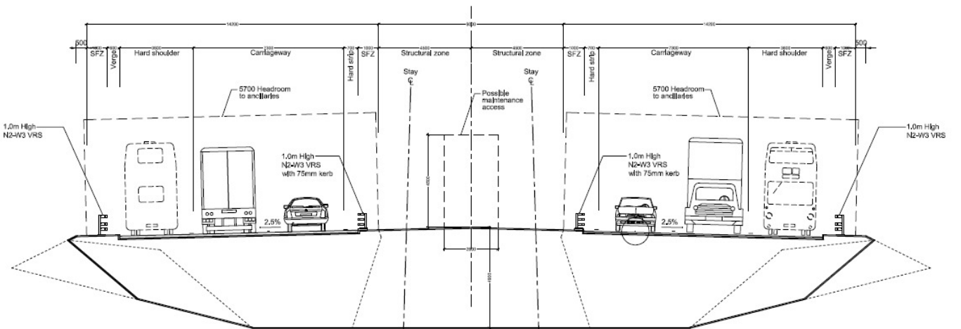
Cable Stay Deck at Transition
