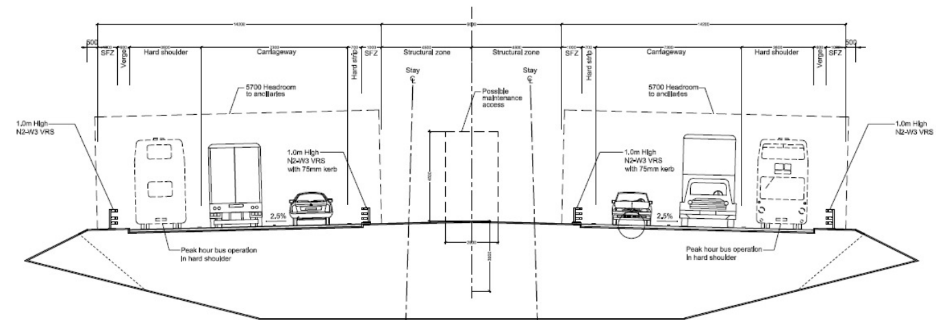
Cable Stay Deck at Main Span
