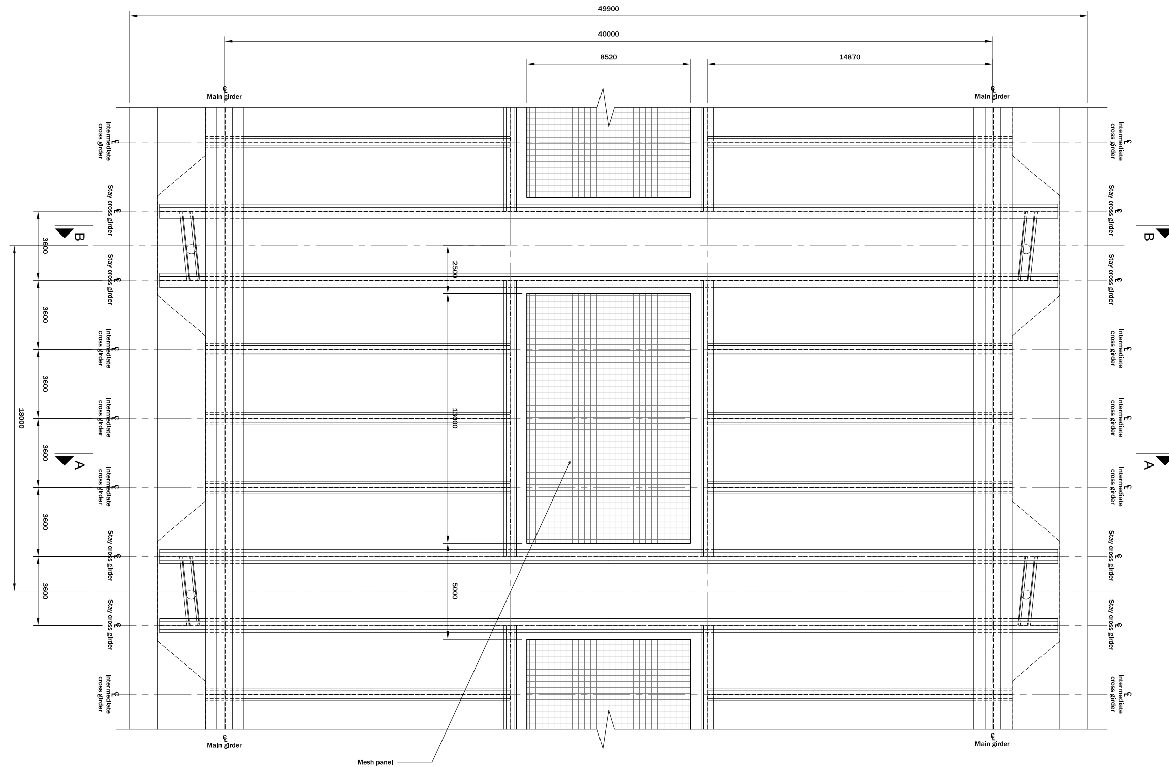
TWIN DECK - TYPICAL PLAN ON VENTED BAY
