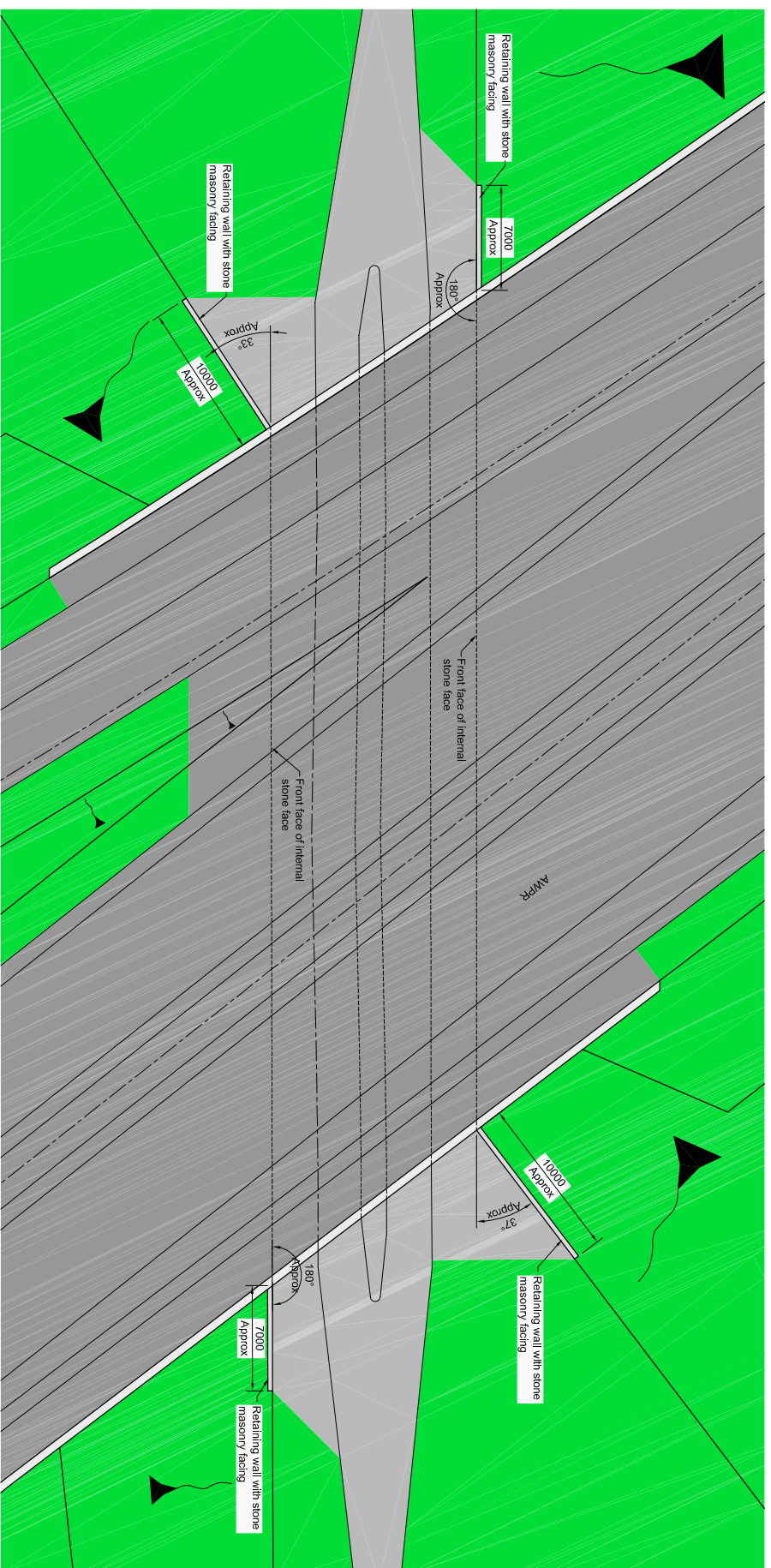
Plan on PS55 Scale 1:200
