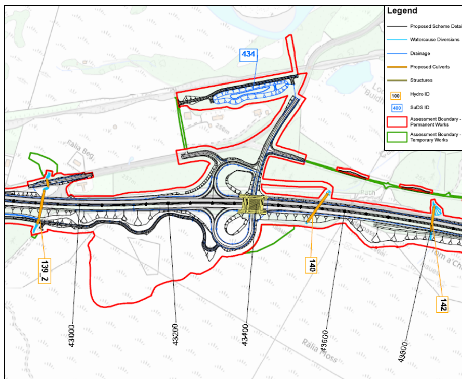
Figure 6-1: Overview of Permanent and Temporary Works assessment boundaries approach
