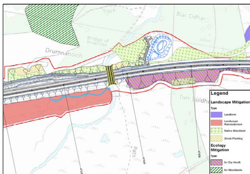
Figure 6-2: Overview of identification of land required for mitigation approach
