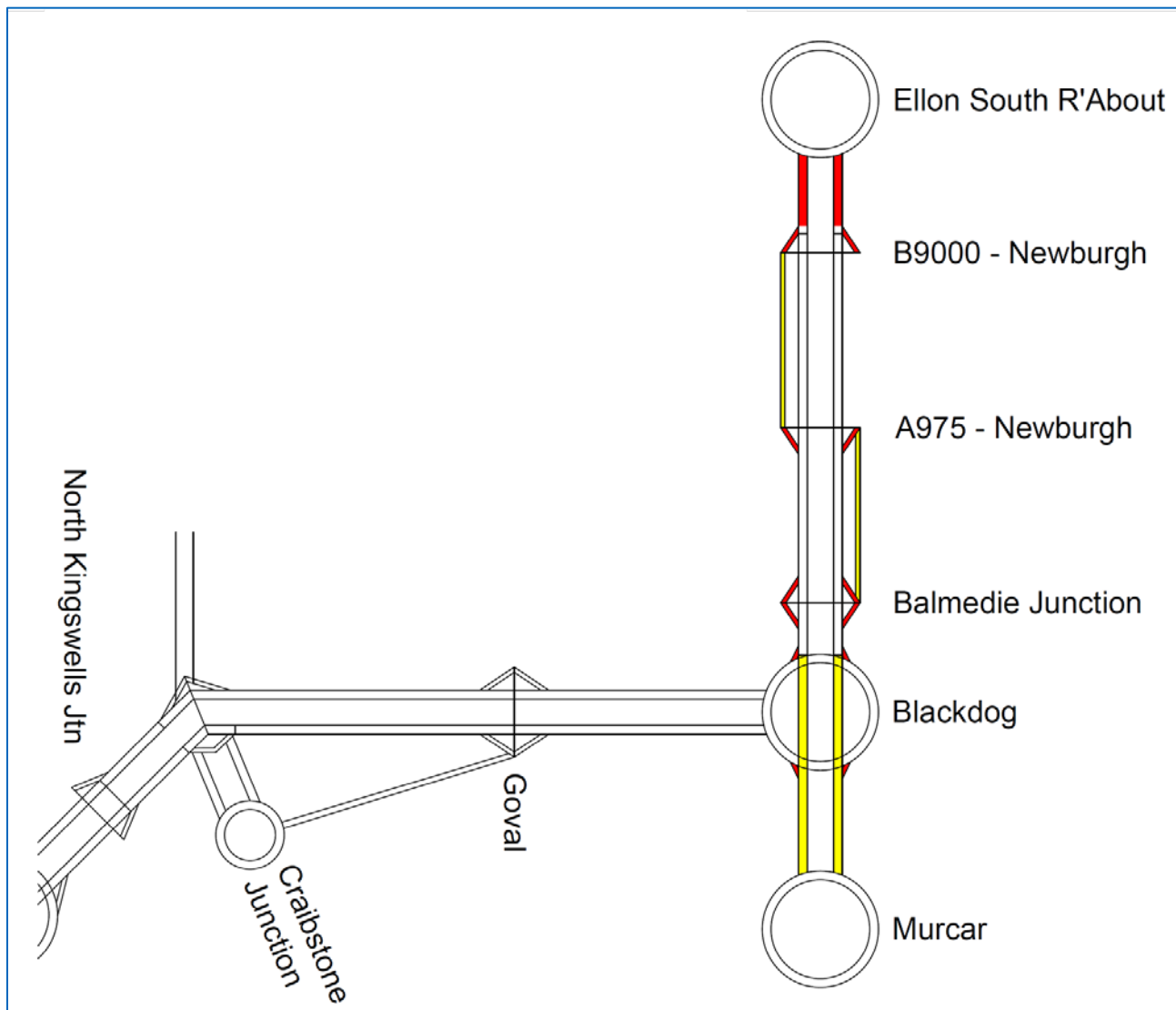
Schematic: Route 5, Ellon to Parkhill Junction (slips) and Restricted Services Network
