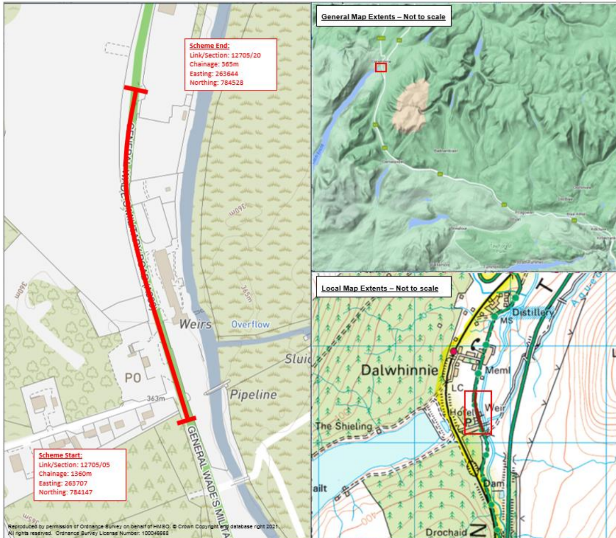
Figure 1. Location and scheme extent of the proposed resurfacing works at A889 Dalwhinnie. Source: BEAR Scotland. F108 – Environmental Assessment Request (Scheme ref: 22-NW-0103-22). Alt text included.
