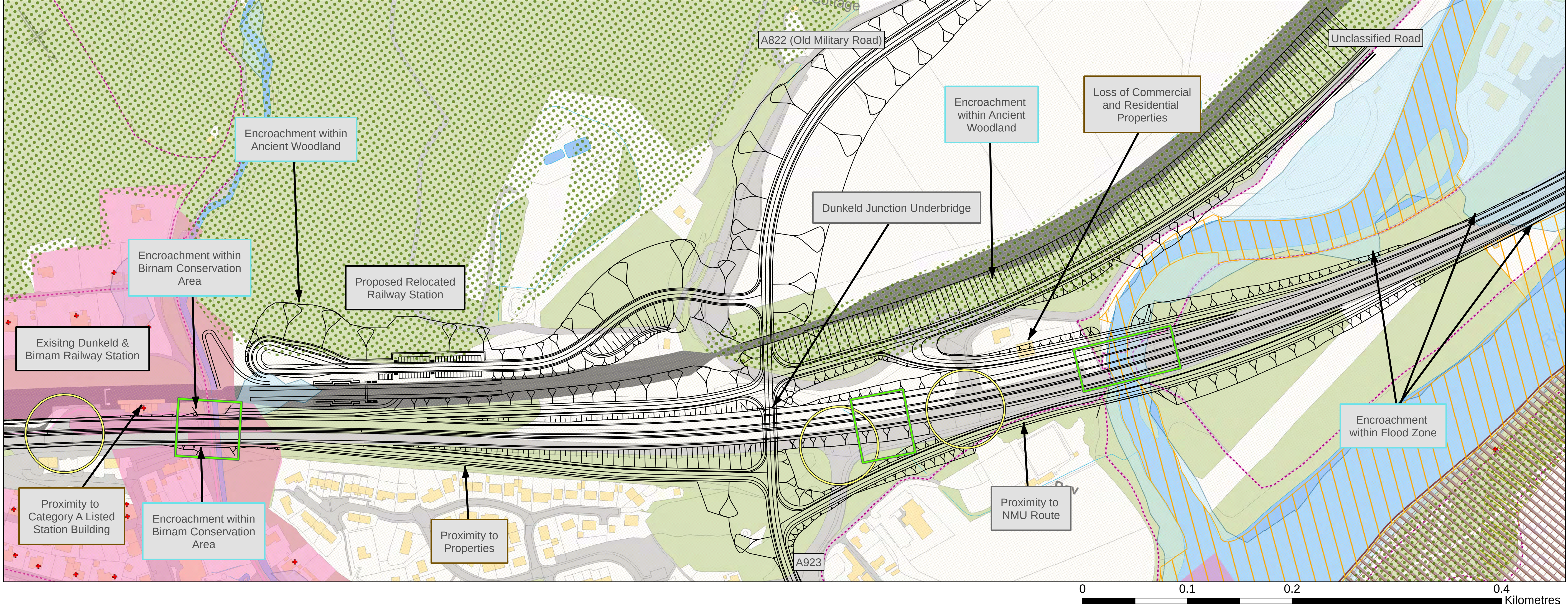
DUNKELD JUNCTION - OPTION C
