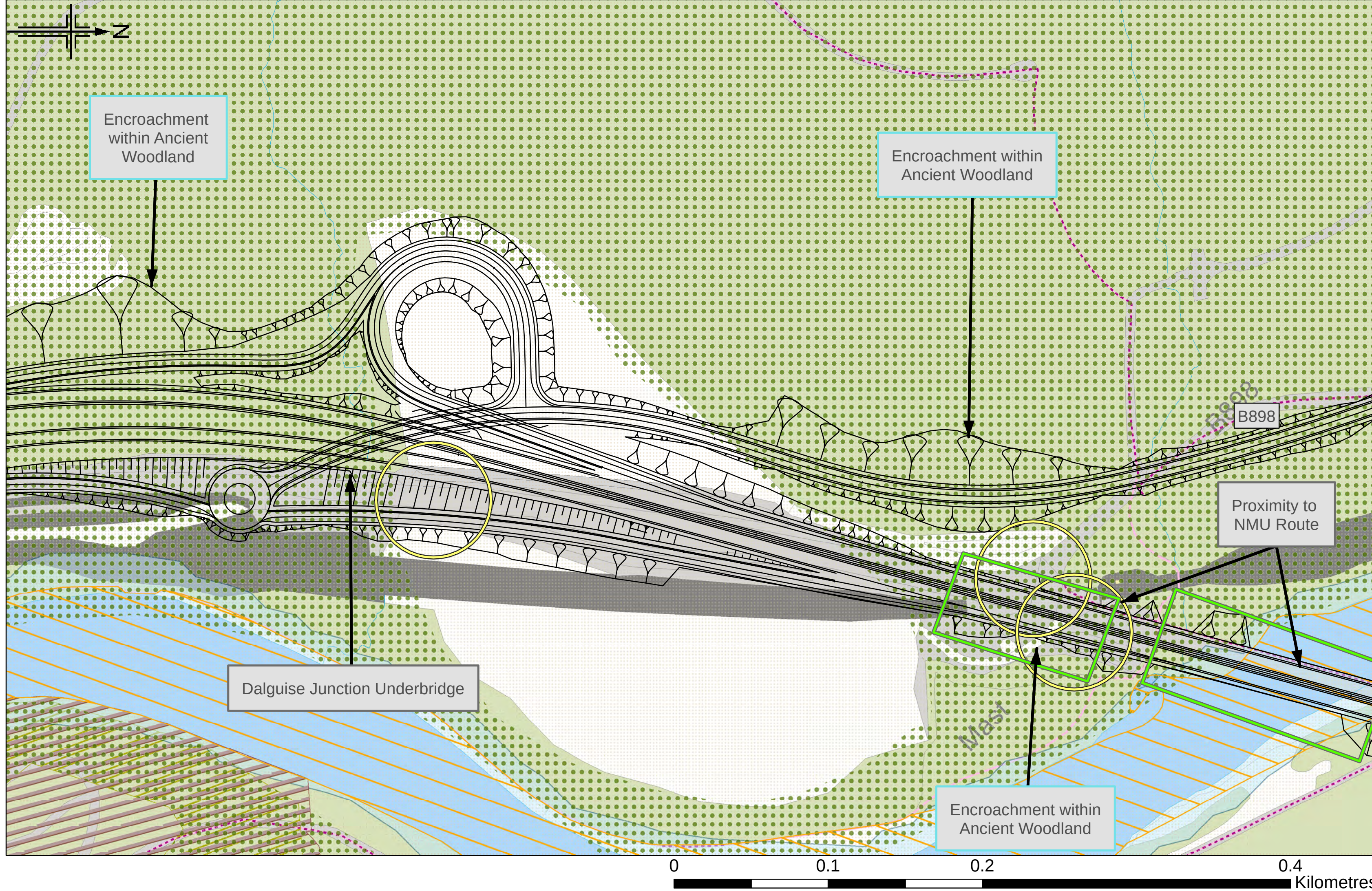
DALGUISE JUNCTION - OPTION C
