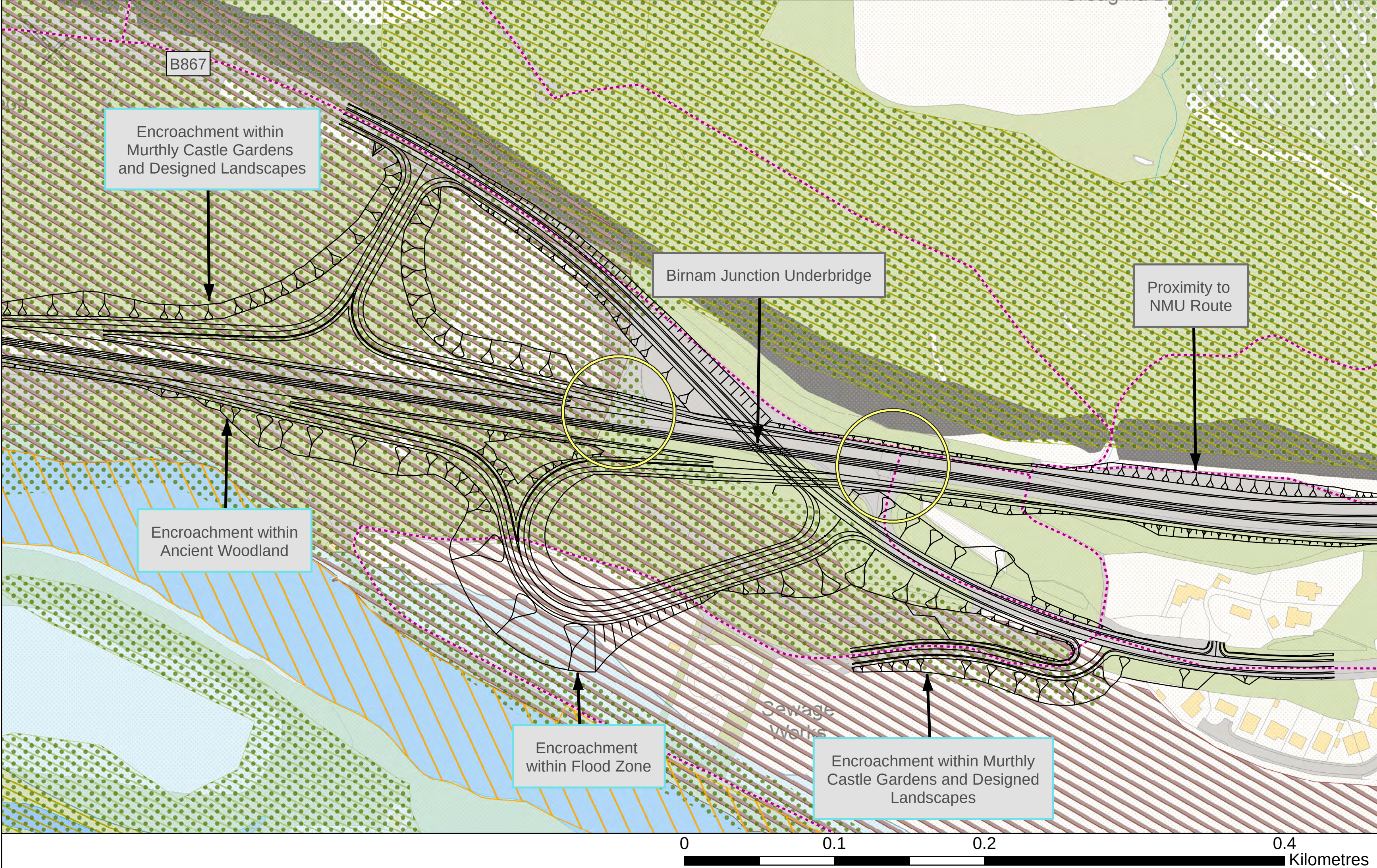
BIRNAM JUNCTION - OPTION C
