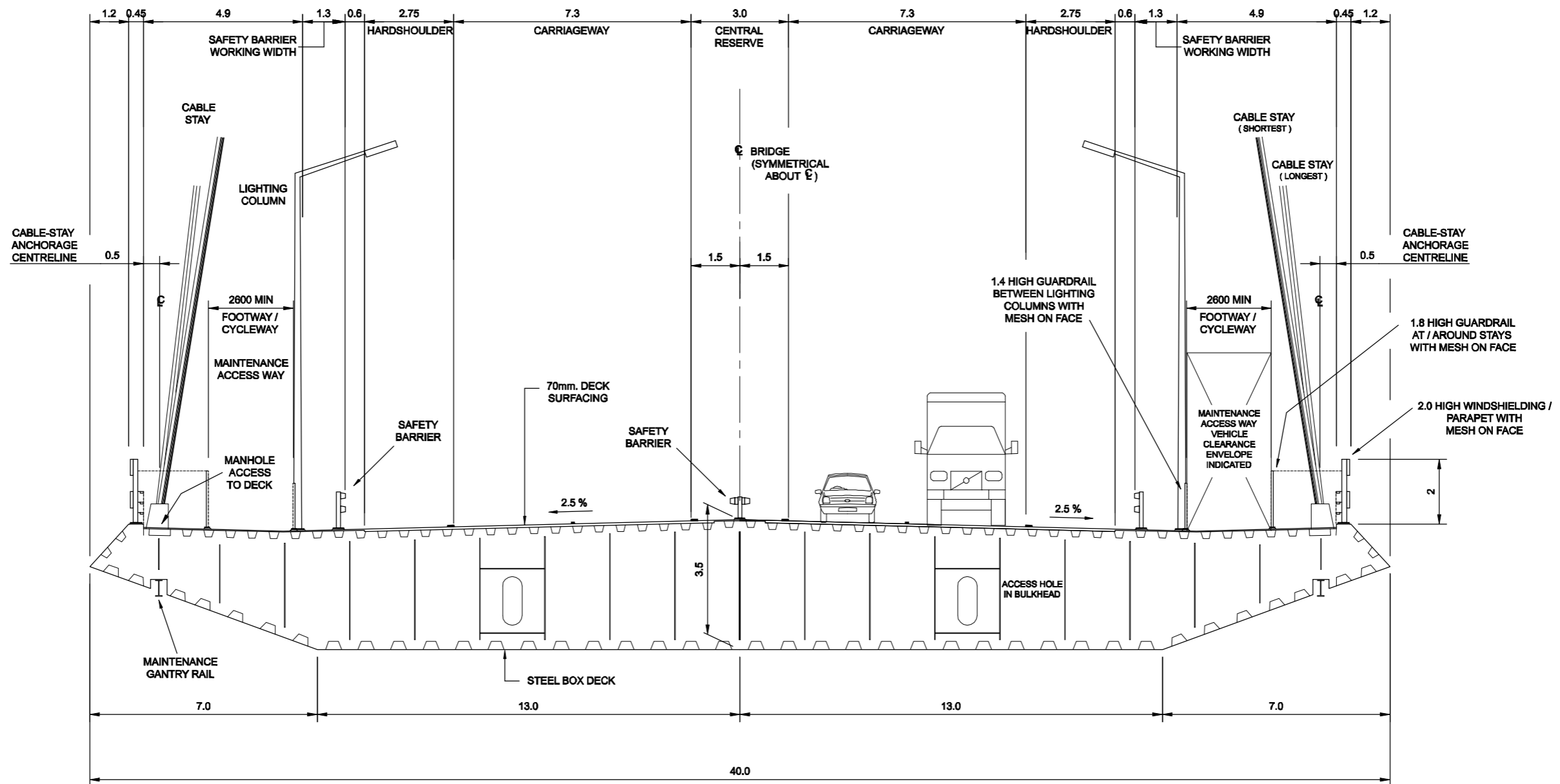
CROSS SECTION THROUGH BRIDGE DECK SCALE 1:150
