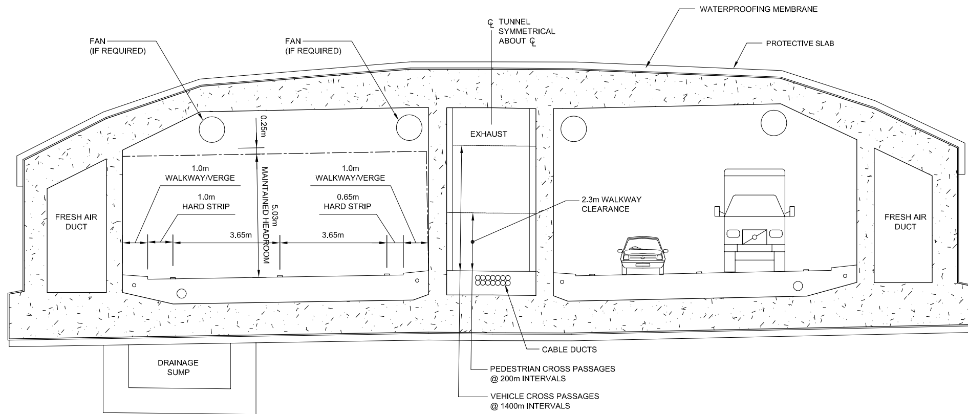
CROSS SECTION THROUGH IMMERSERD TUBE TUNNEL SCALE 1:150
