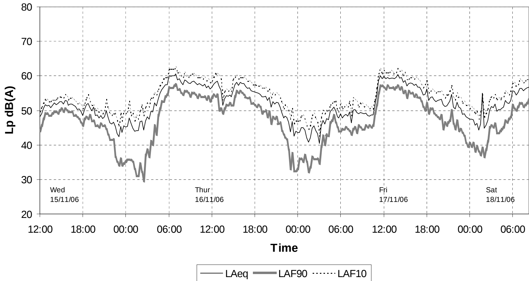
M4 Tarbolton Road Ambient Noise Levels
