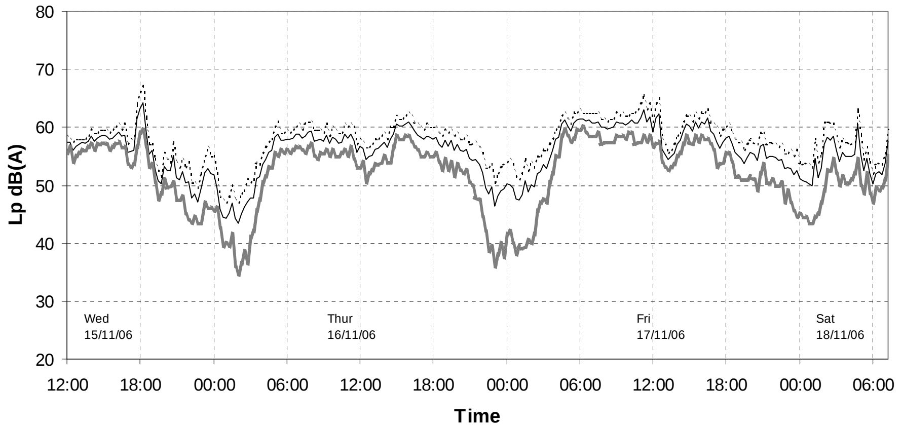
M3 Stockbridge Cottage Monitored Noise Levels
