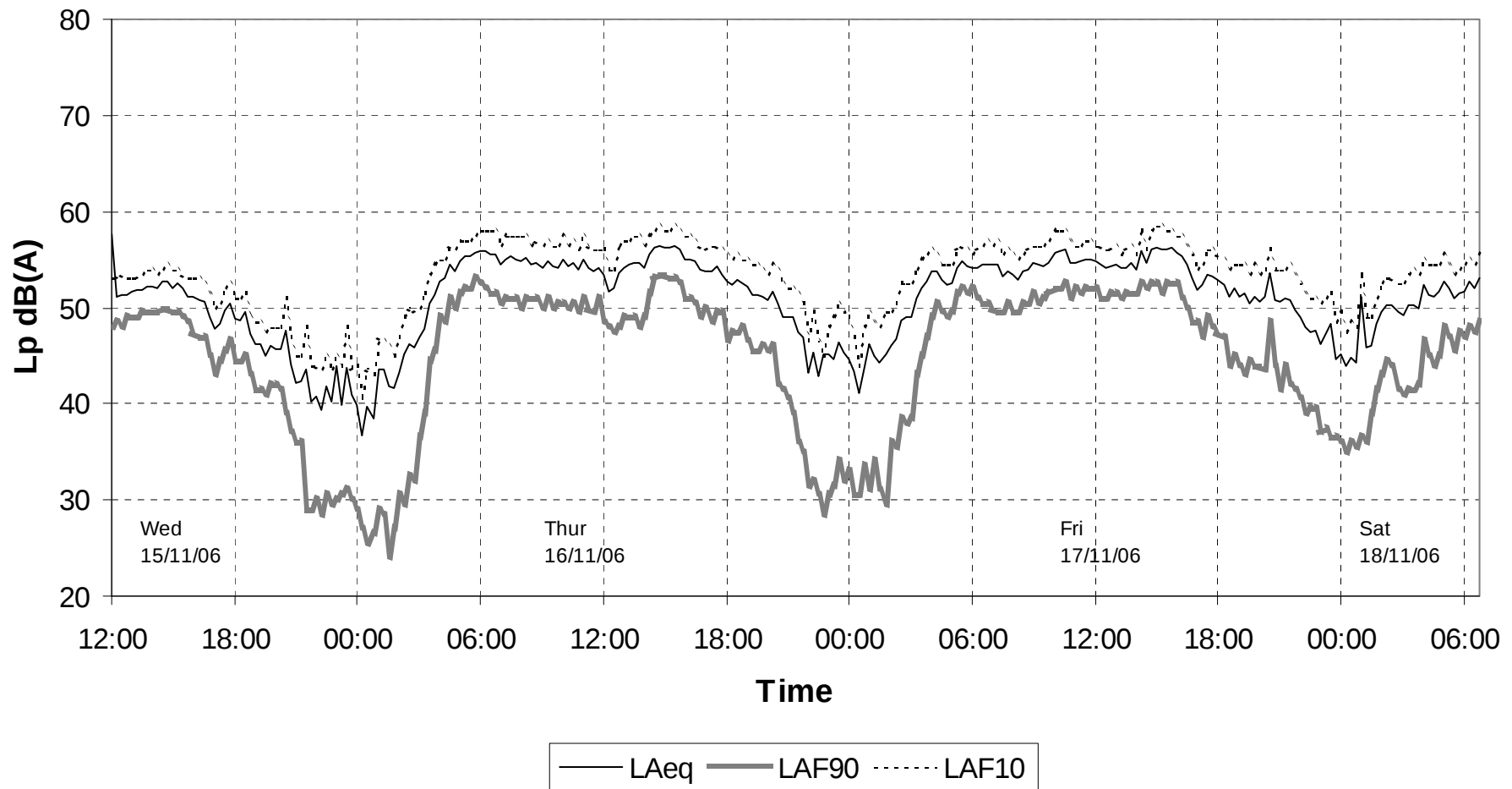
M2 South Trynlow Cottage Ambient Noise Levels
