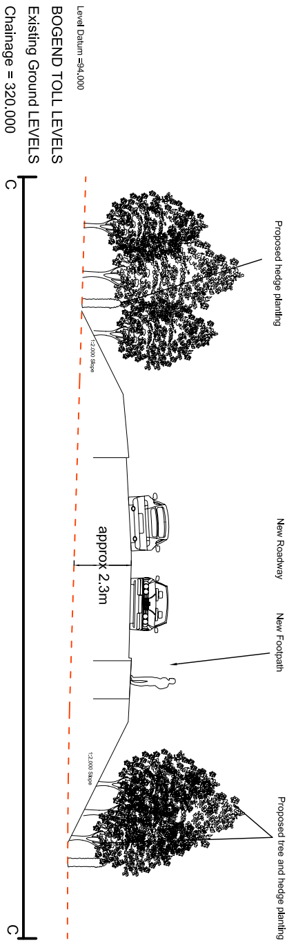
Section BB, for approximate section location refer to Figure 2.3 Sheet 5 of 6. Scale : 1:100 at A3
