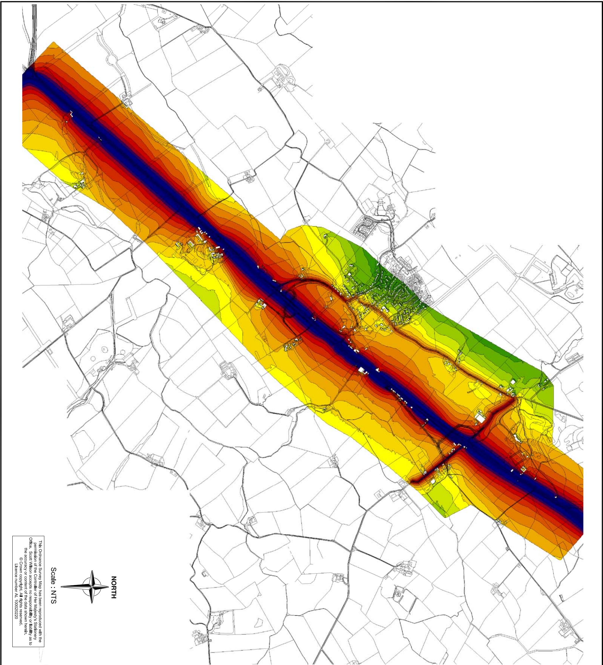
FIGURE 9.6 2024 Baseline - Traffic Noise Levels
