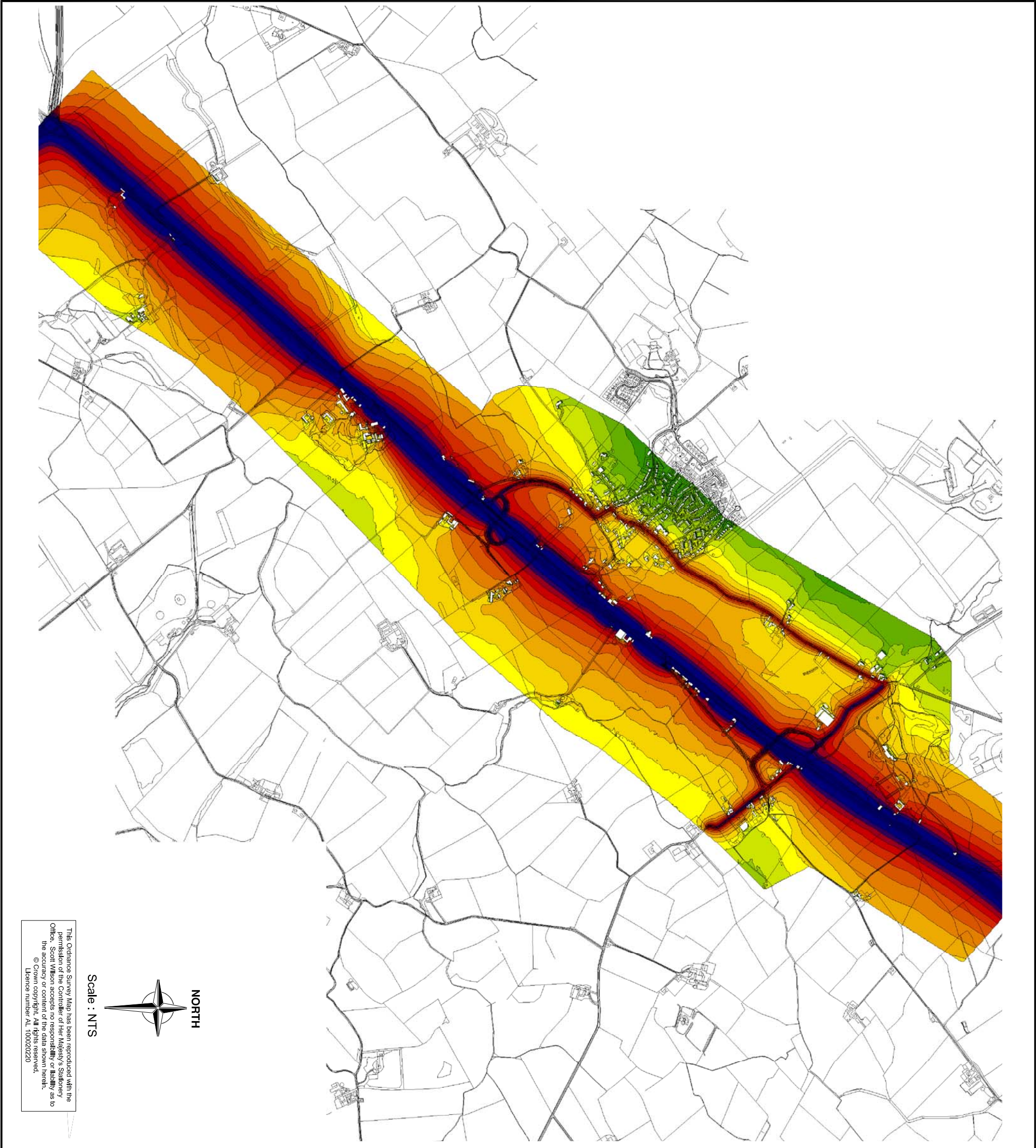
FIGURE 9.8 2024 With Scheme - Traffic Noise Levels
